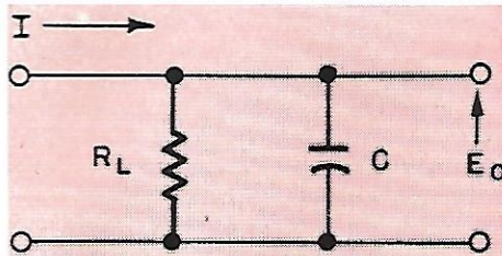
Figure 2. Load shunted by parasitic capacity, usually specified. The existence of one without the other, however, indicates a non-linear phase delay and is wasteful since the build-up time is not minimized.
