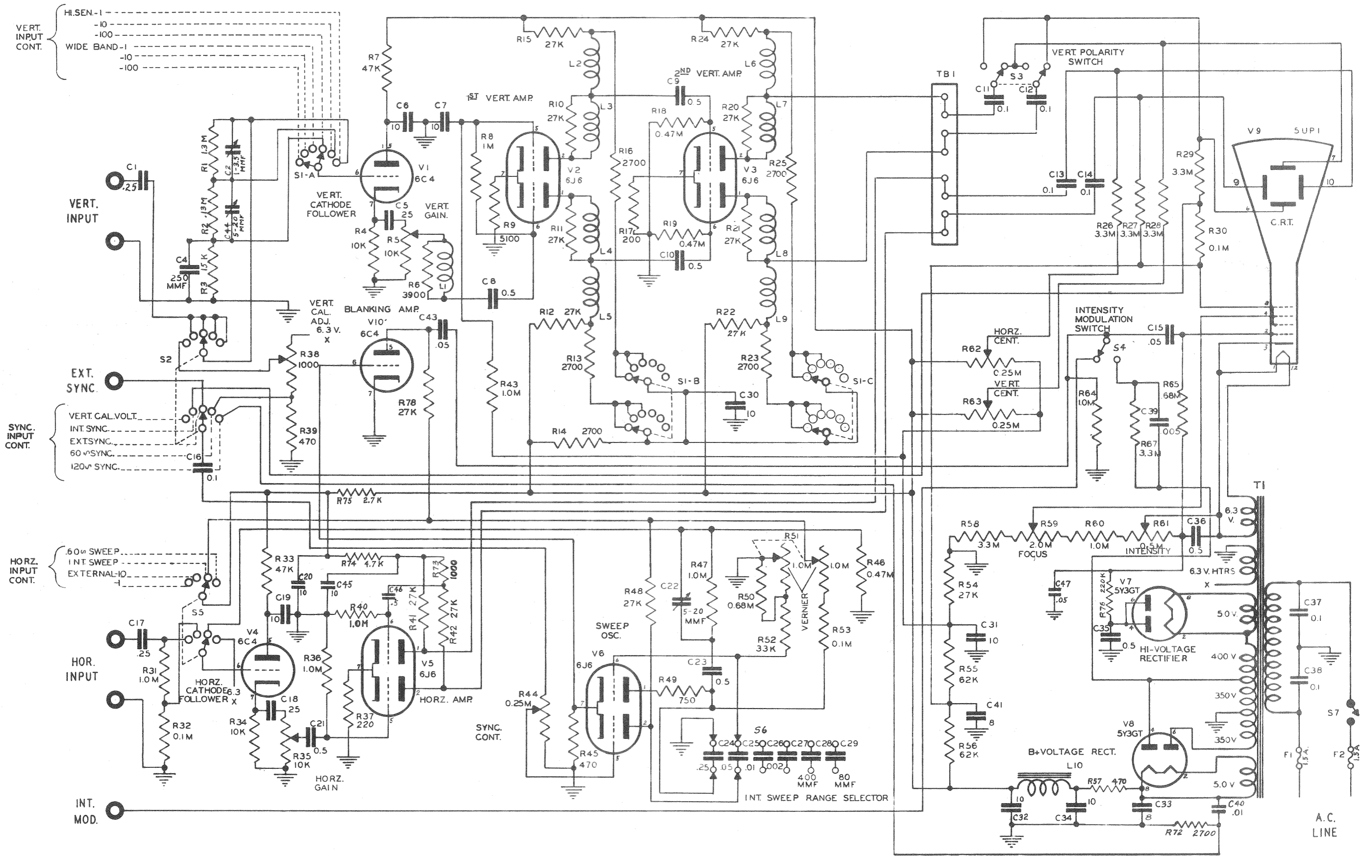
Schematic Diagram Model CRO-2 Drawing No. C-499B R2755
