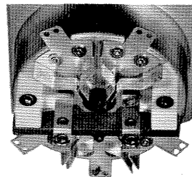
Bottom View of Socket Showing R-F By-Pass Condensers
