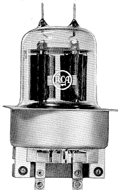
Socket with Tube in Position
