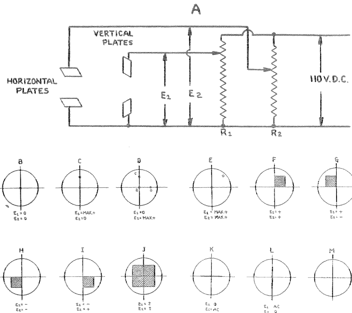
Figure 4—Application of Voltage to Deflecting Plates
