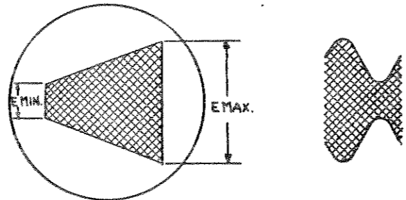
Timing Axis Supply—The Modulating Signal Percent Modulation = \frac{EM_{\max} - E_{\min}}{EM_{\max} + E_{\min}} \times 100
