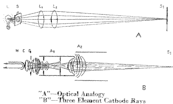
Figure 2—Focusing Cathode Rays
