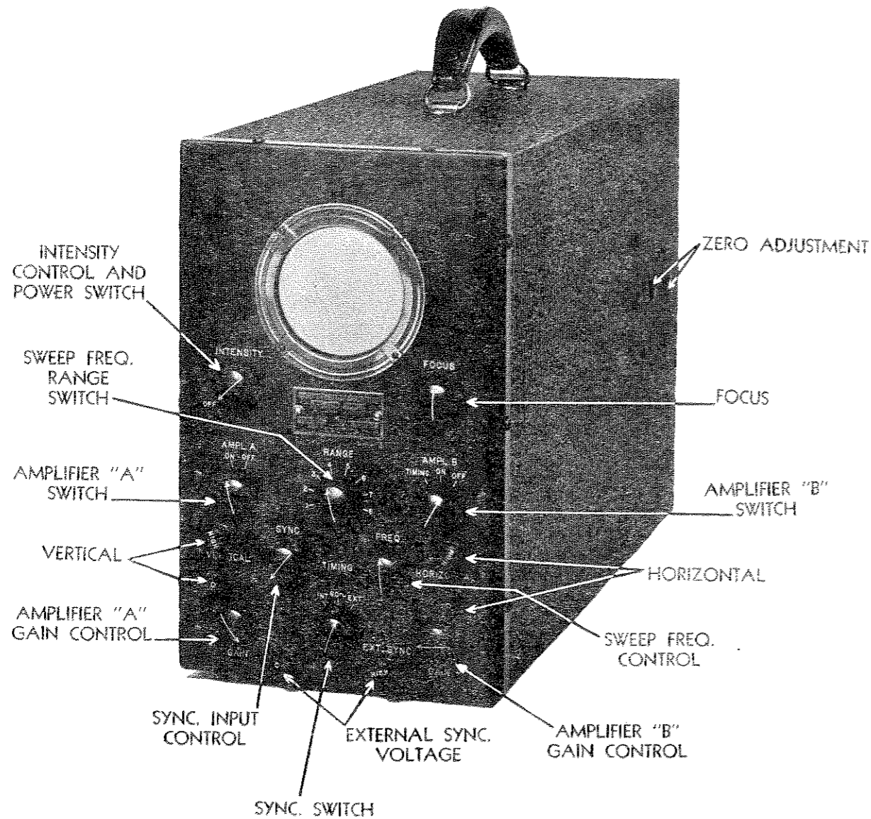
Frontispiece—Front View of Cathode-Ray Oscilloscope, Type TMV-122-B
