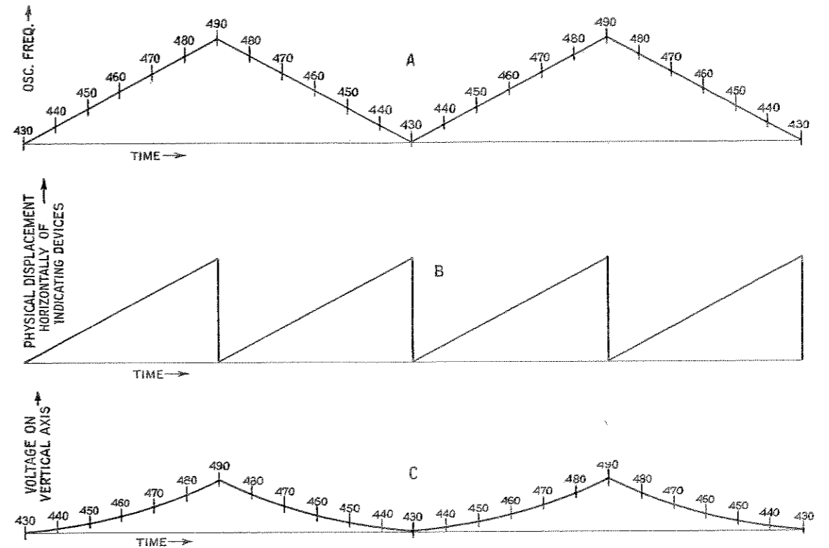
NOTE: C is the resultant curve when the signal of A is fed into a circuit with characteristics of D. With signal B on the horizontal plates and C on the vertical plates, E is the resultant image on the screen.
