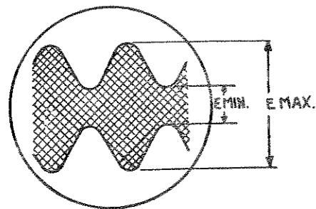
R. F. Modulated at 1000 Cycles Timing Axis Supply: 500-Cycle Saw-Tooth Percent Modulation = \frac{EM_{\max} - E_{\min}}{EM_{\max} + E_{\min}} \times 100
